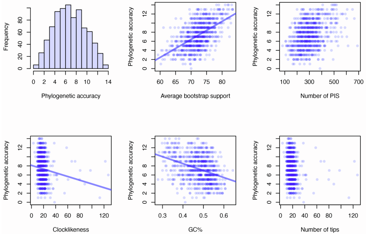
Figure S1. Frequency distribution of phylogenetic accuracy scores of the loci used for phylogenetic reconstructions of bees (Apoidea: Apiformes). Related to Figure 1, Table S1, and to the STAR Methods. The 830 UCE loci of the set filtered for 75% taxonomic completeness were categorized according to their phylogenetic accuracy scores; frequency distribution and relationships with five potential correlates; regression lines are shown for the three significant correlations found.
